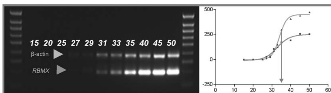
Figure 3. Saturation curve for both the study and control gene. A number of cycles corresponding to the exponential phase of the reaction for both genes was chosen.
